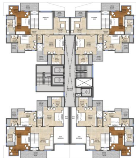
3 BHK+3T+SERVANT PENTHOUSE TOWER PLAN AT UPPER LEVEL
