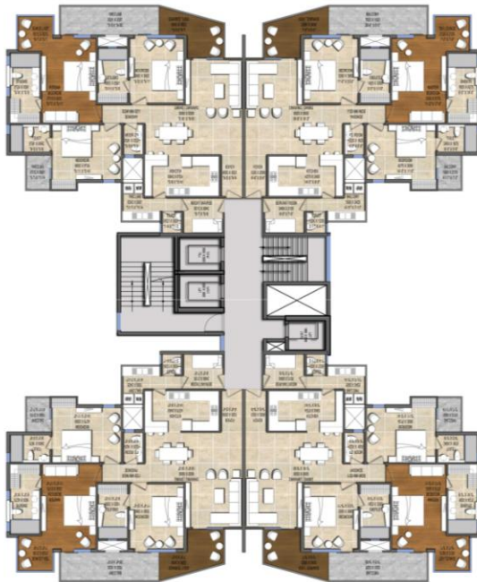
3 BHK+3T+SERVANT TYPICAL FLOOR PLAN
